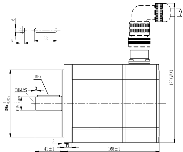
Mechanical View 7
