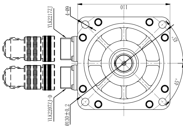
Mechanical View 6
