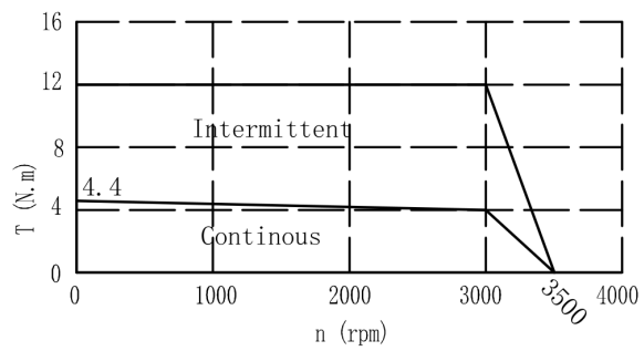
Mechanical View 9
