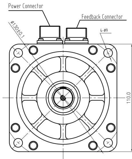
Mechanical View 7
