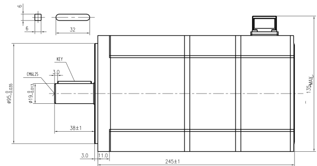
Mechanical View 8
