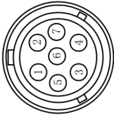
Mechanical View 3
