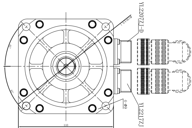
Mechanical View 5
