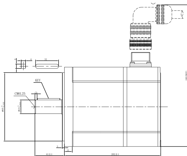
Mechanical View 6
