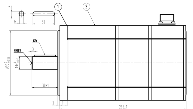
Mechanical View 8
