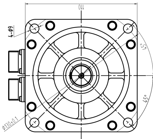
Mechanical View 7
