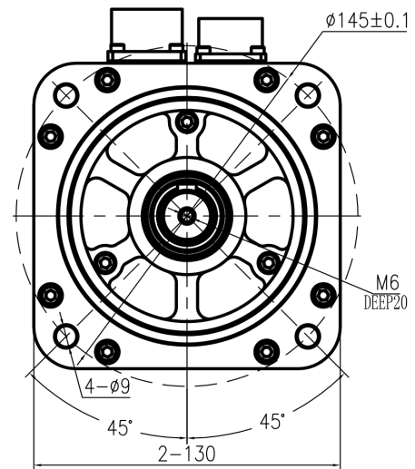
Mechanical View 7
