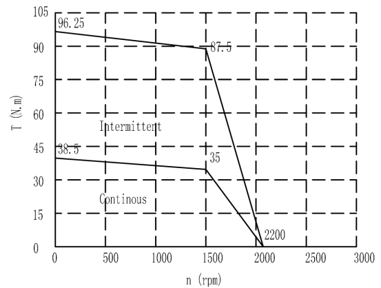
Mechanical View 8
