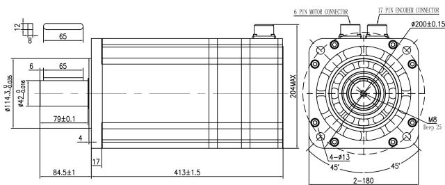
Mechanical View 7
