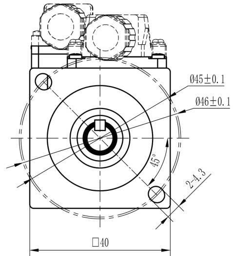
Mechanical View 2
