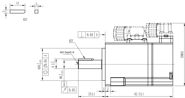
Mechanical View 1
