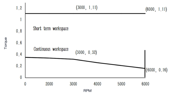
Mechanical View 10
