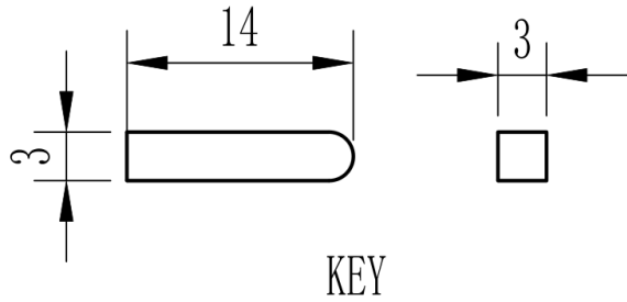
Mechanical View 1
