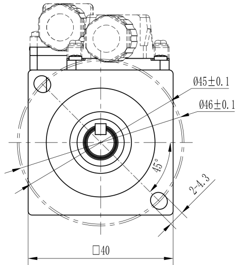
Mechanical View 3
