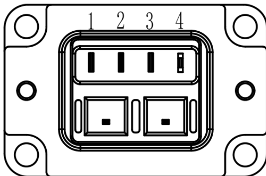
Mechanical View 4
