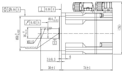
Mechanical View 1
