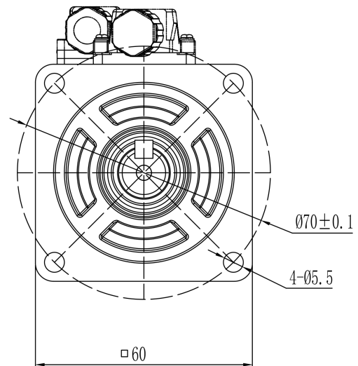
Mechanical View 2
