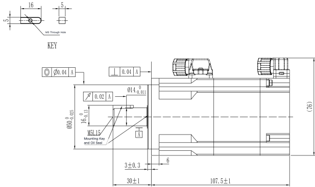
Mechanical View 1
