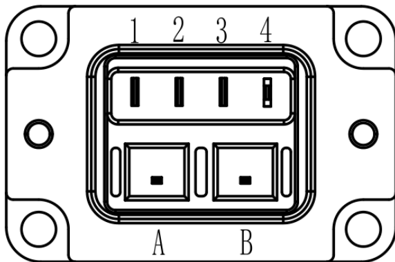
Mechanical View 5
