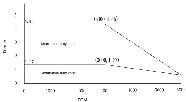
Mechanical View 9
