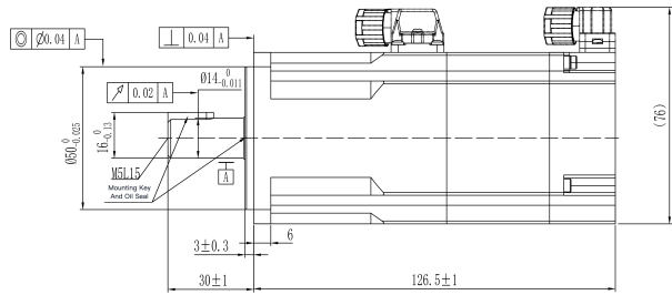
Mechanical View 1
