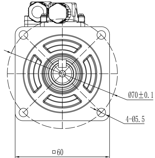
Mechanical View 2
