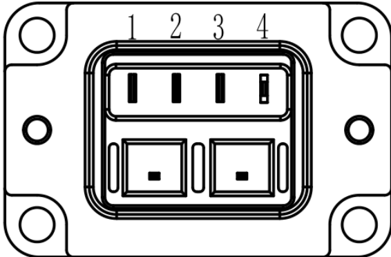
Mechanical View 5
