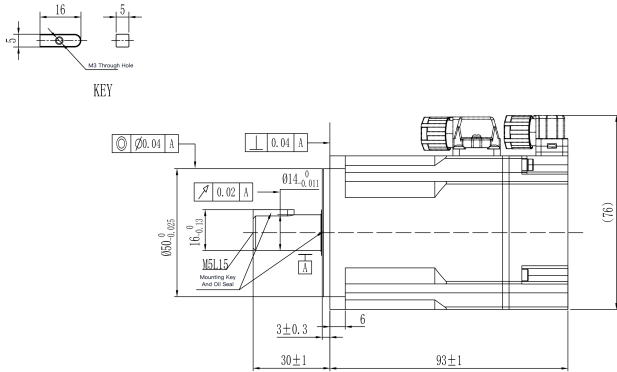
Mechanical View 1
