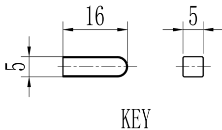
Mechanical View 3
