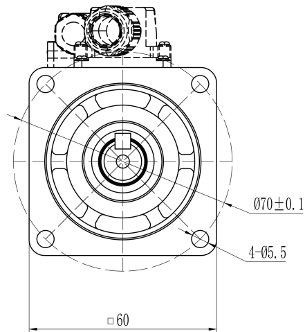
Mechanical View 1
