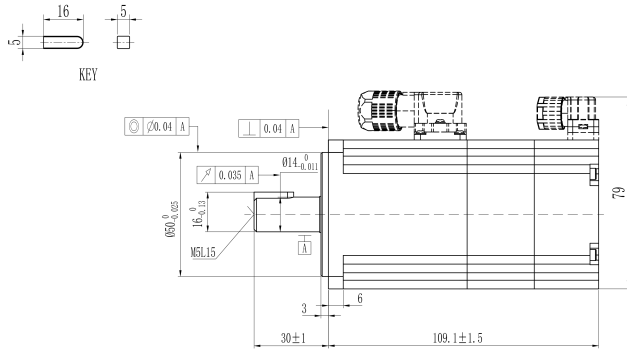
Mechanical View 1
