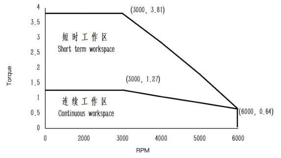
Mechanical View 10
