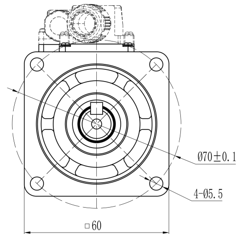
Mechanical View 2
