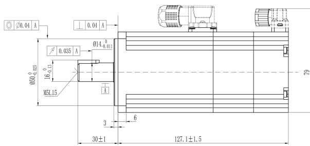
Mechanical View 3
