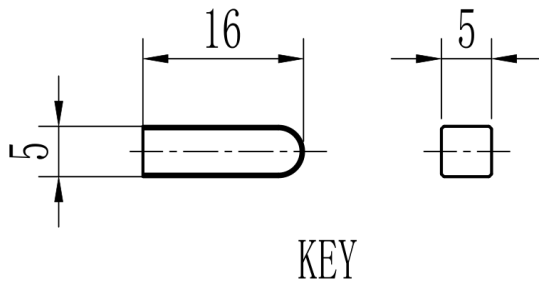
Mechanical View 1
