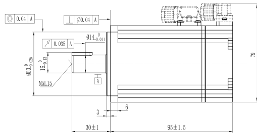
Mechanical View 1
