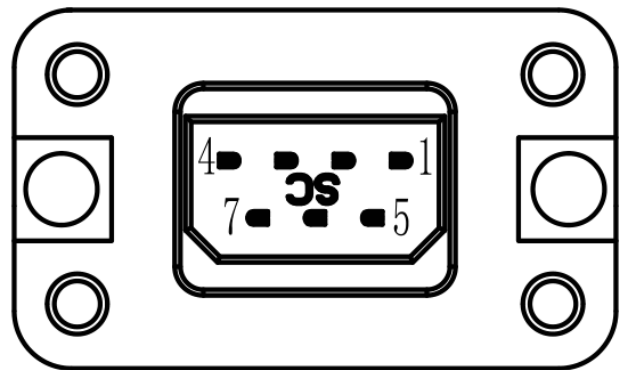
Mechanical View 2
