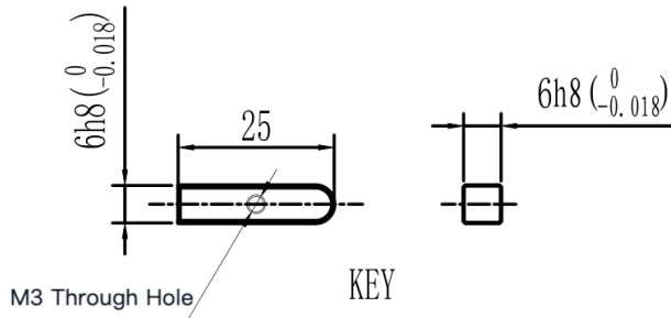
Mechanical View 1
