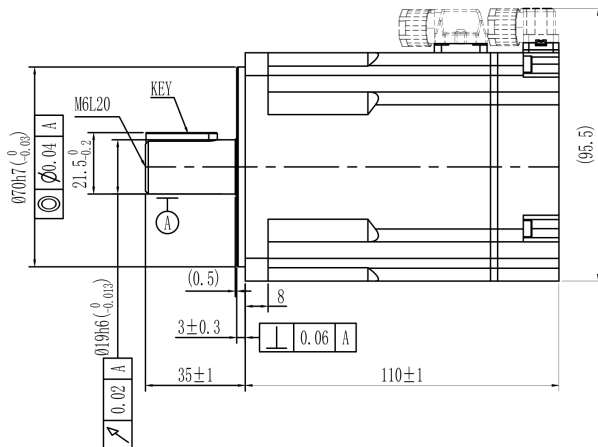
Mechanical View 3
