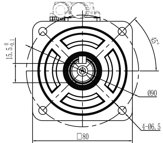
Mechanical View 2
