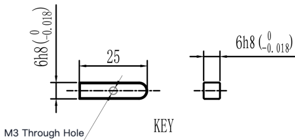
Mechanical View 3
