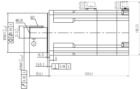
Mechanical View 2
