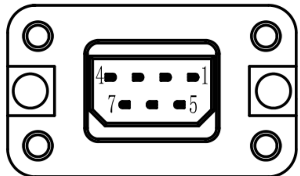
Mechanical View 9
