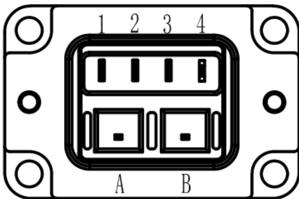
Mechanical View 5
