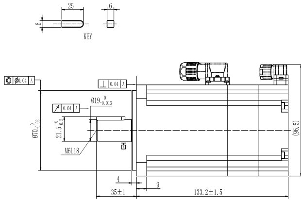
Mechanical View 1
