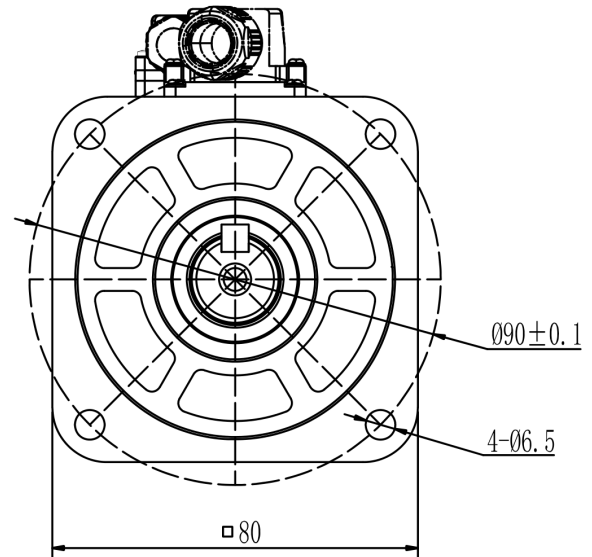
Mechanical View 2
