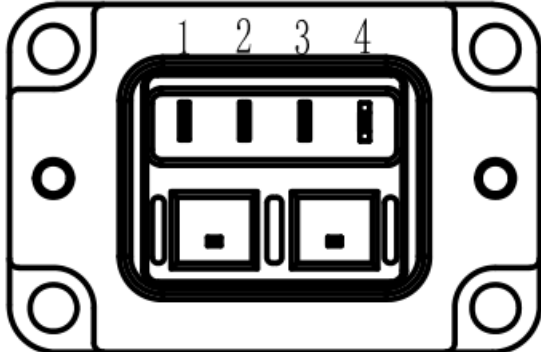
Mechanical View 5
