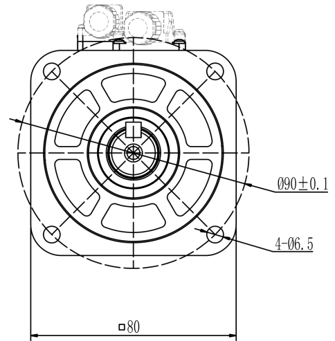
Mechanical View 2
