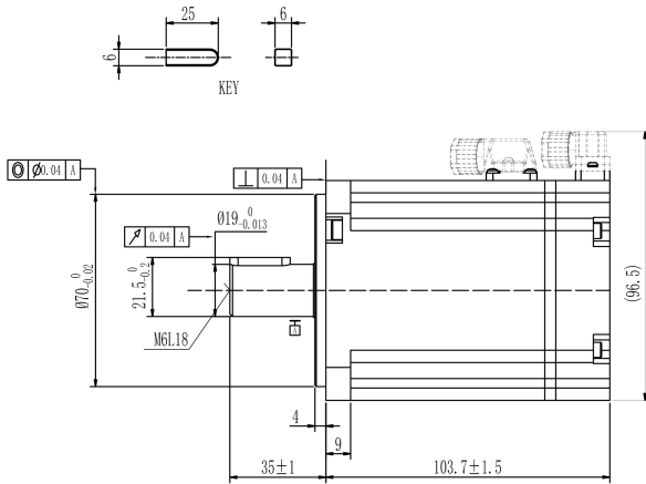
Mechanical View 1
