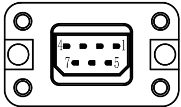
Mechanical View 9
