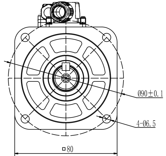
Mechanical View 2
