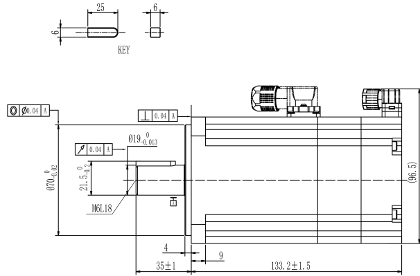
Mechanical View 1
