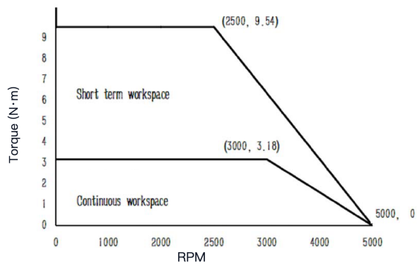
Mechanical View 11
