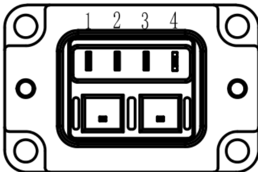
Mechanical View 5
