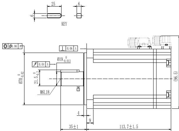
Mechanical View 1
