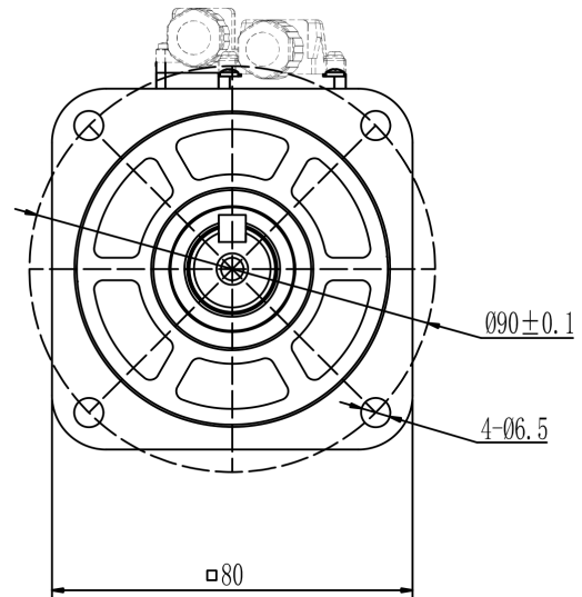
Mechanical View 2
