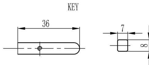
Mechanical View 1
