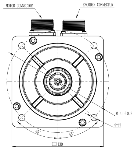
Mechanical View 2
