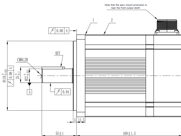
Mechanical View 3
