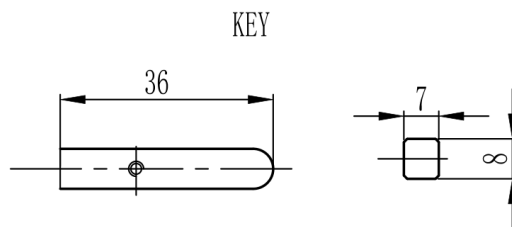
Mechanical View 1
