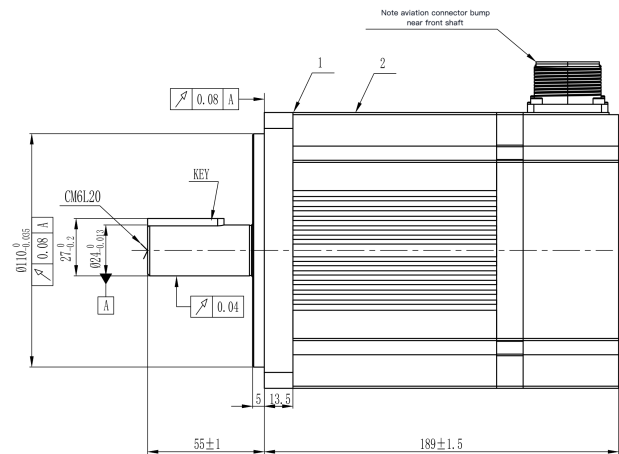
Mechanical View 2
