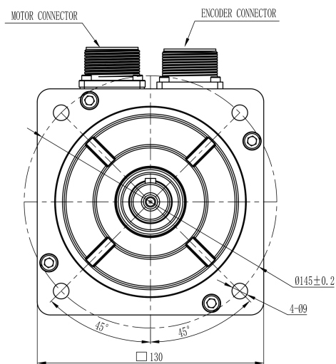
Mechanical View 3
