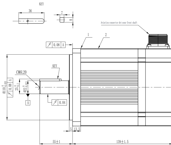
Mechanical View 1
