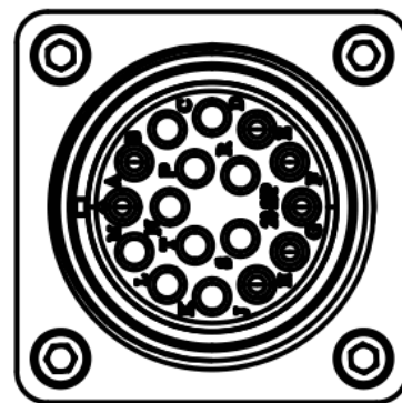
Mechanical View 6
