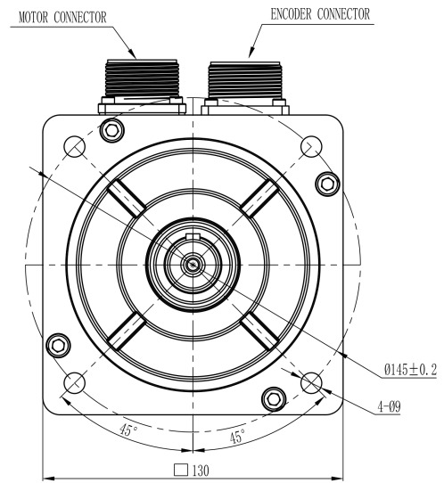
Mechanical View 2
