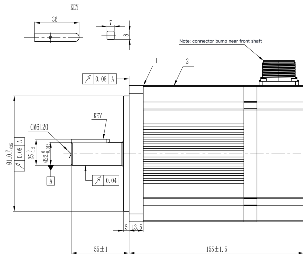
Mechanical View 1
