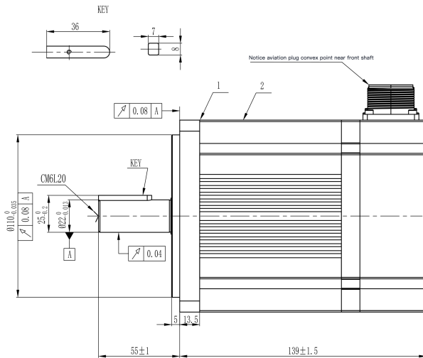
Mechanical View 1
