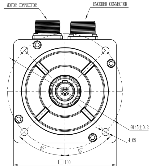
Mechanical View 2
