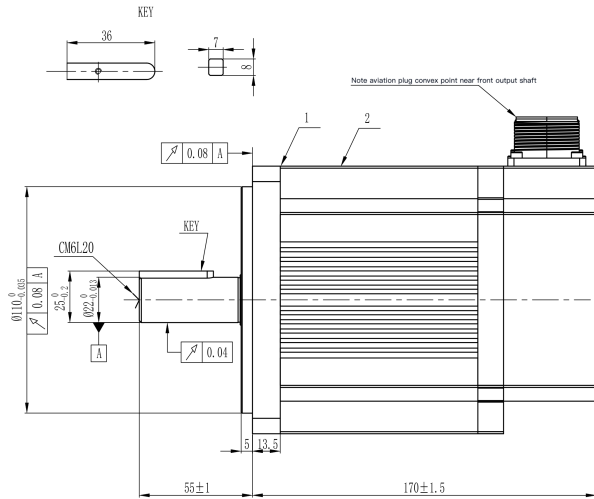
Mechanical View 1
