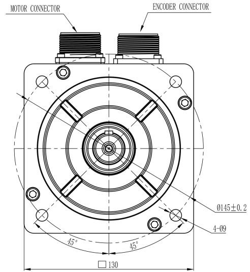
Mechanical View 2
