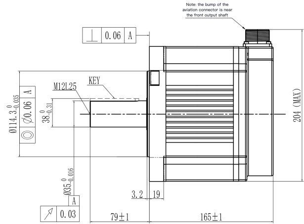
Mechanical View 2
