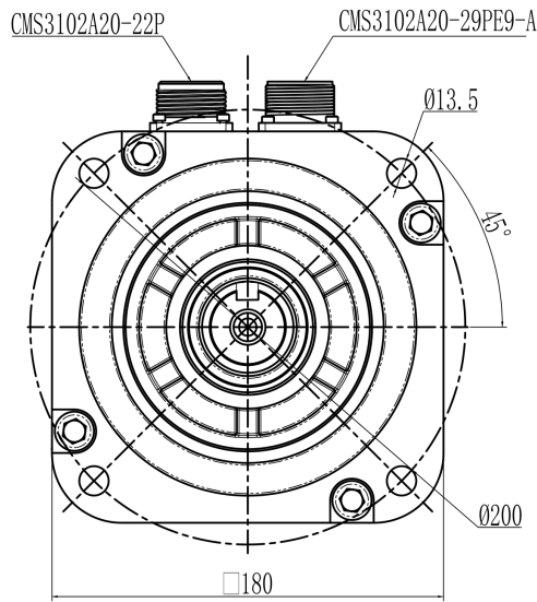
Mechanical View 1
