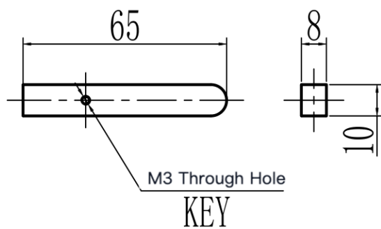
Mechanical View 3
