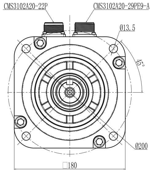
Mechanical View 1
