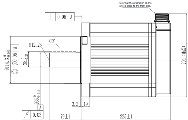
Mechanical View 2
