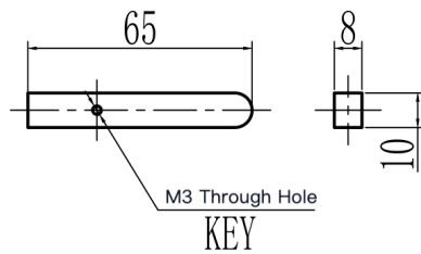
Mechanical View 3
