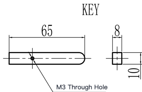
Mechanical View 3
