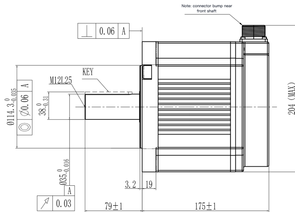
Mechanical View 1
