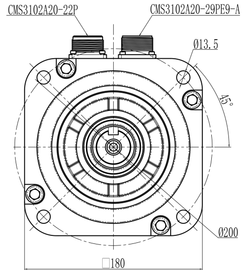
Mechanical View 2
