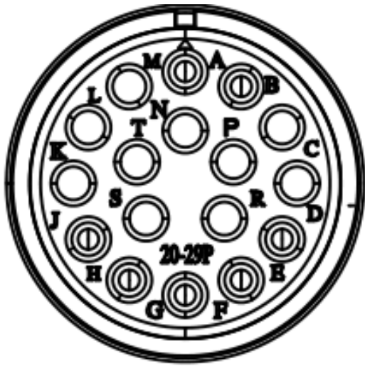
Mechanical View 8
