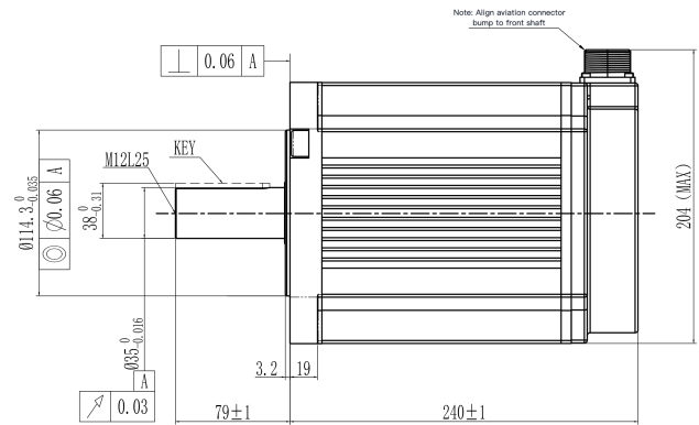
Mechanical View 2
