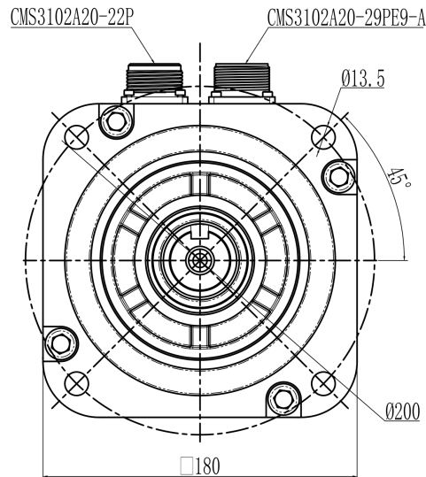
Mechanical View 1
