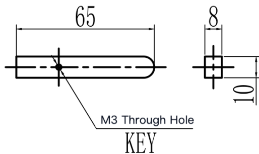
Mechanical View 3
