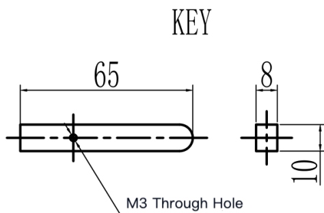
Mechanical View 3
