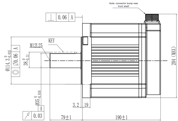
Mechanical View 2
