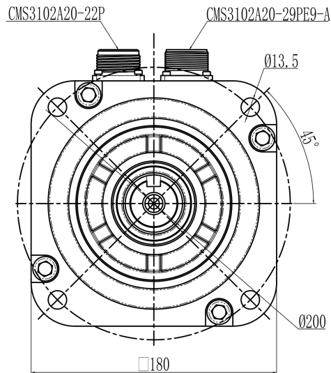
Mechanical View 1
