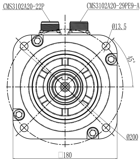
Mechanical View 1
