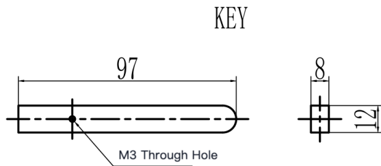
Mechanical View 3
