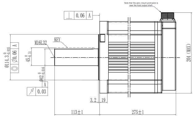
Mechanical View 2
