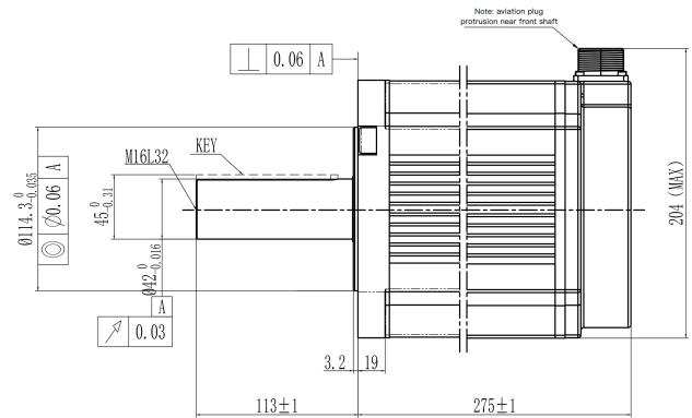
Mechanical View 2
