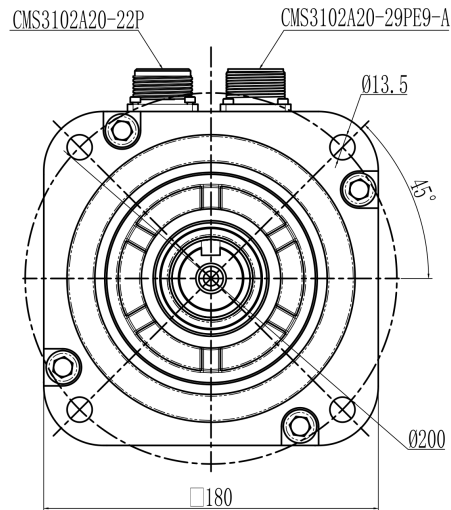
Mechanical View 1
