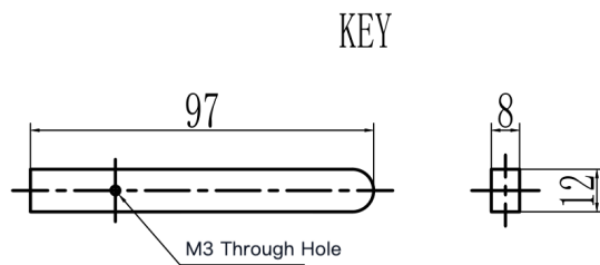
Mechanical View 3
