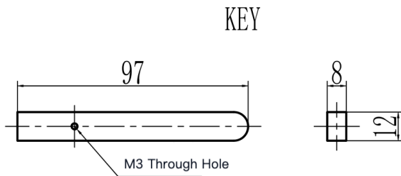
Mechanical View 3
