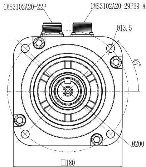
Mechanical View 1
