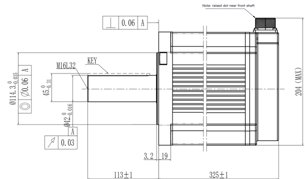
Mechanical View 2
