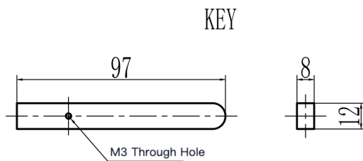
Mechanical View 3
