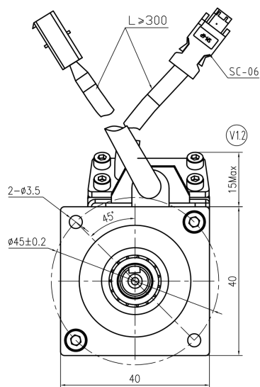
Mechanical View 6
