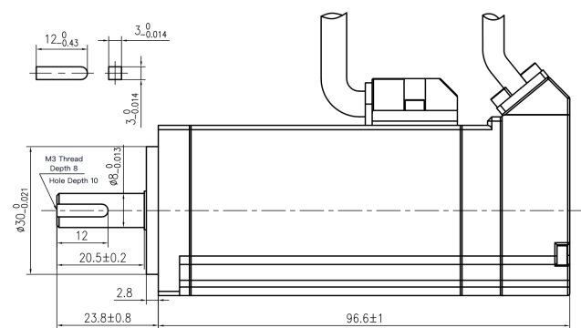
Mechanical View 7
