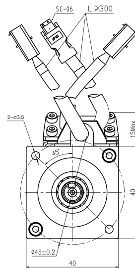
Mechanical View 6
