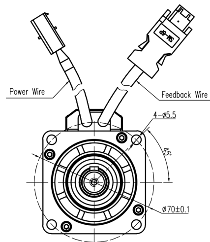
Mechanical View 9
