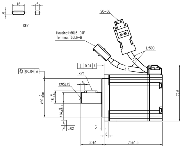
Mechanical View 8
