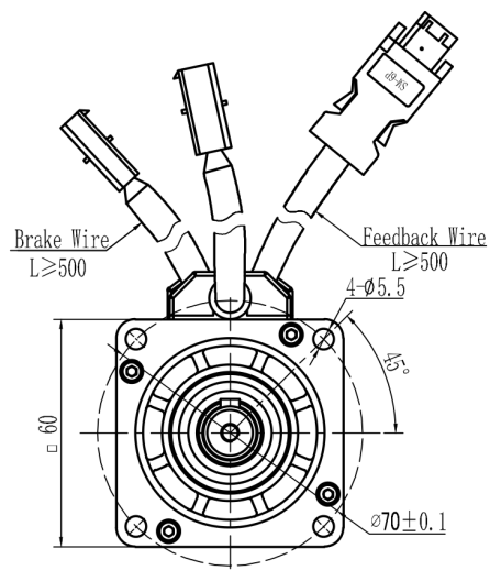
Mechanical View 9
