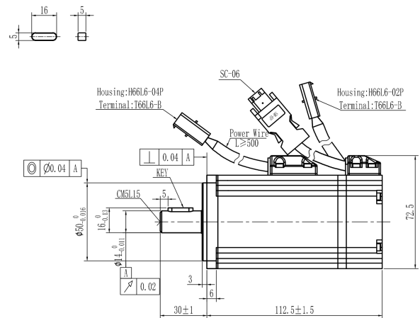
Mechanical View 7
