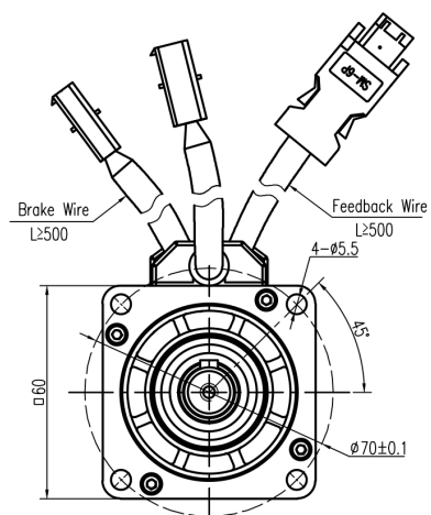
Mechanical View 13
