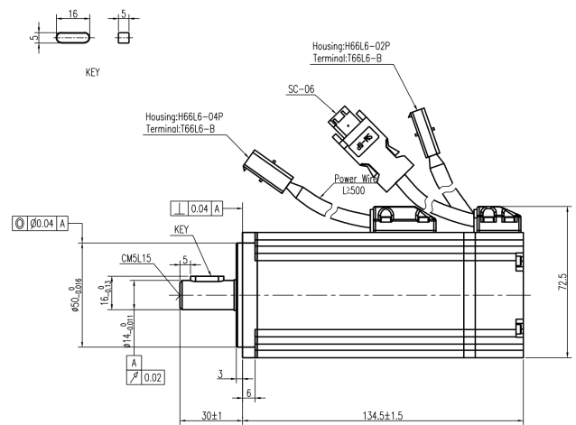
Mechanical View 12
