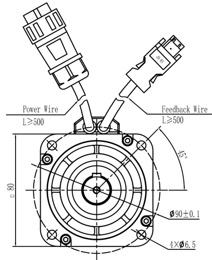
Mechanical View 4
