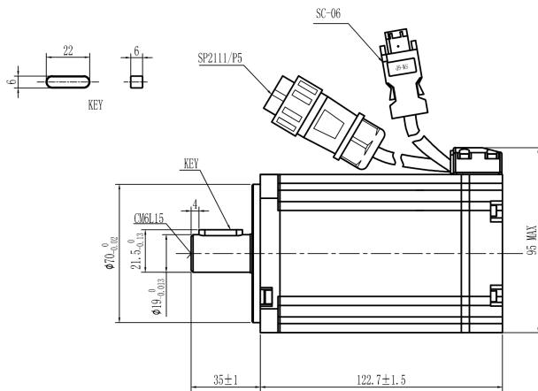
Mechanical View 5
