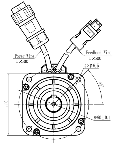
Mechanical View 4
