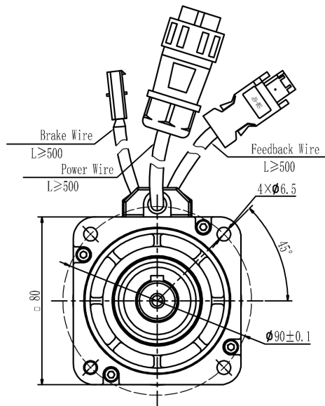
Mechanical View 7
