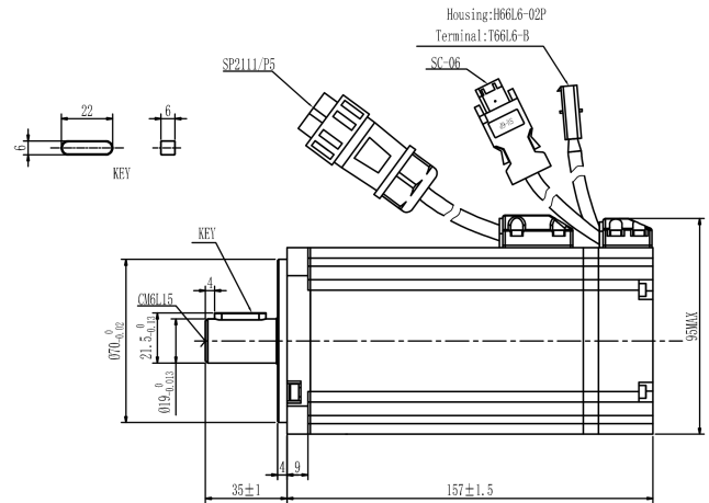
Mechanical View 6
