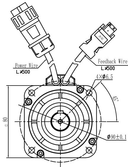
Mechanical View 4
