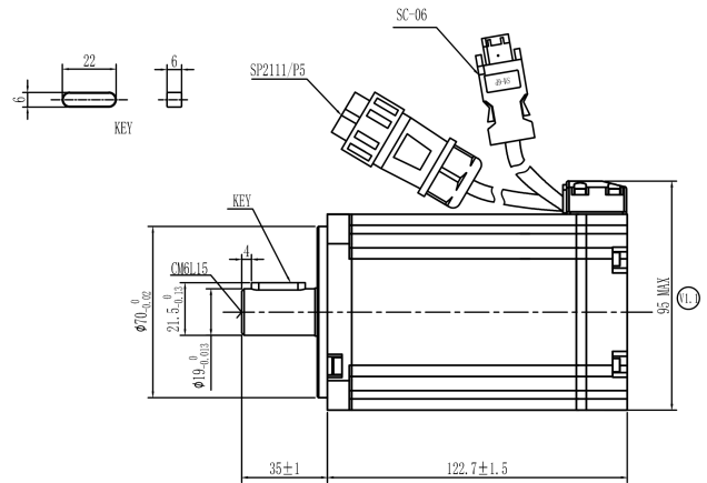
Mechanical View 5
