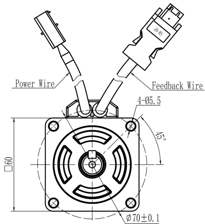
Mechanical View 3
