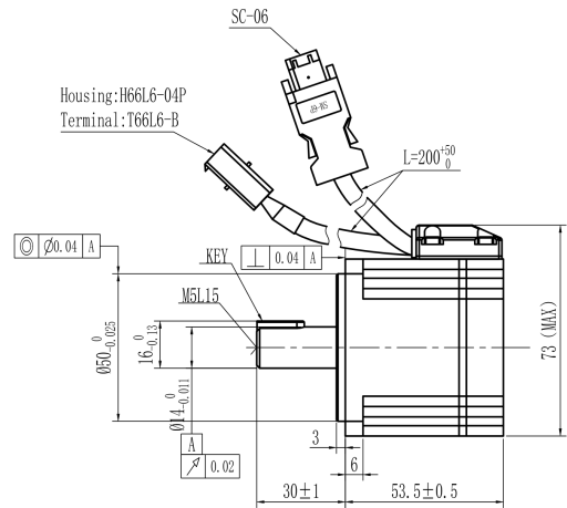
Mechanical View 2
